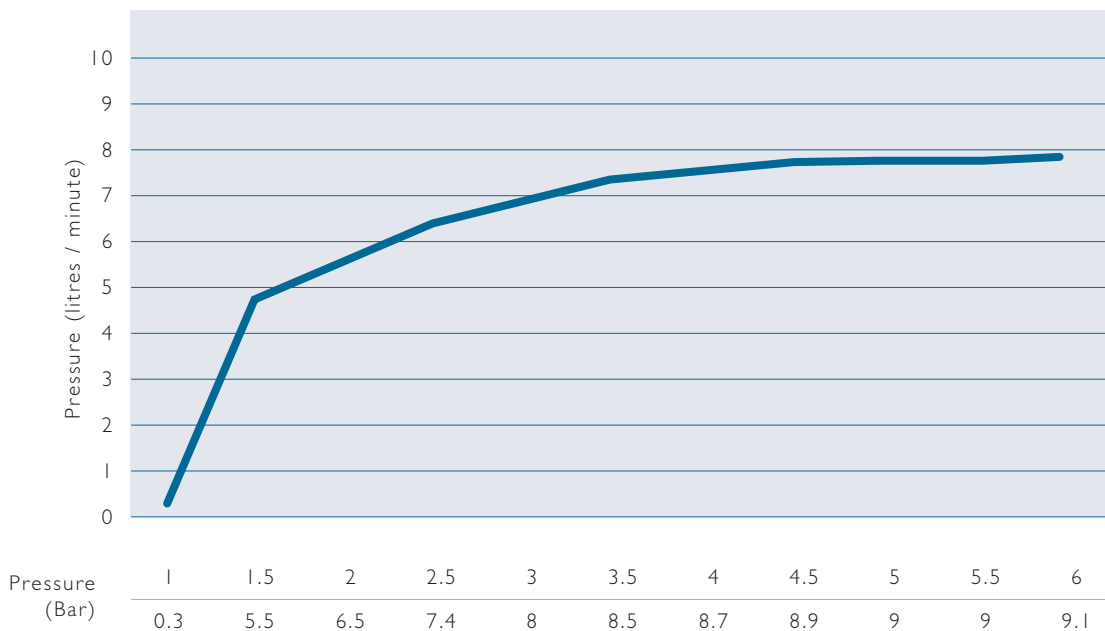
DB3000 Flow rate for 9 litres per minute
